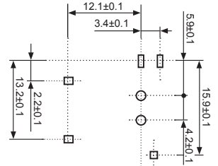
Mounting Hole Layout (Bottom View)
